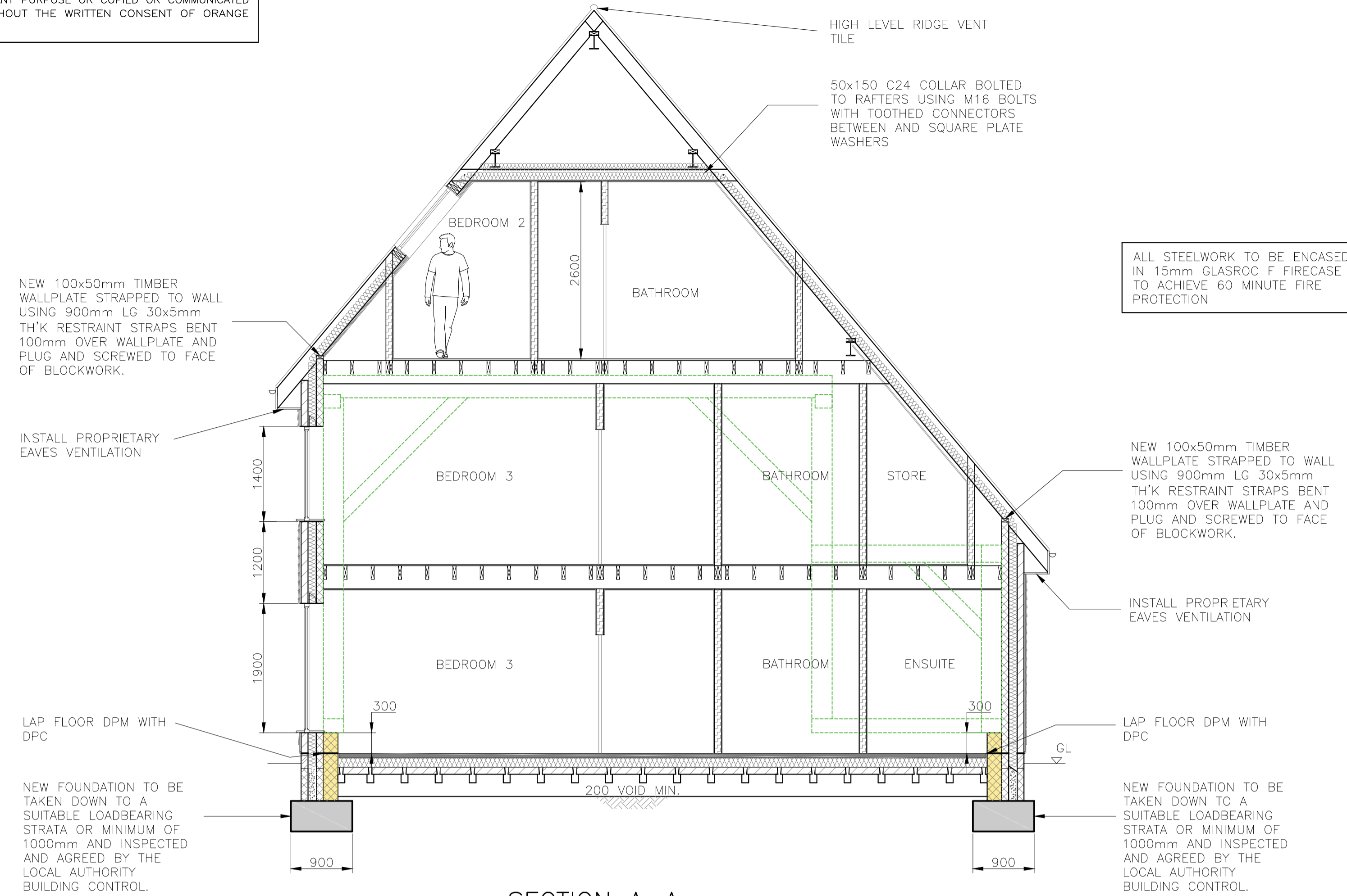
SECTION A-A SCALE 1:50
