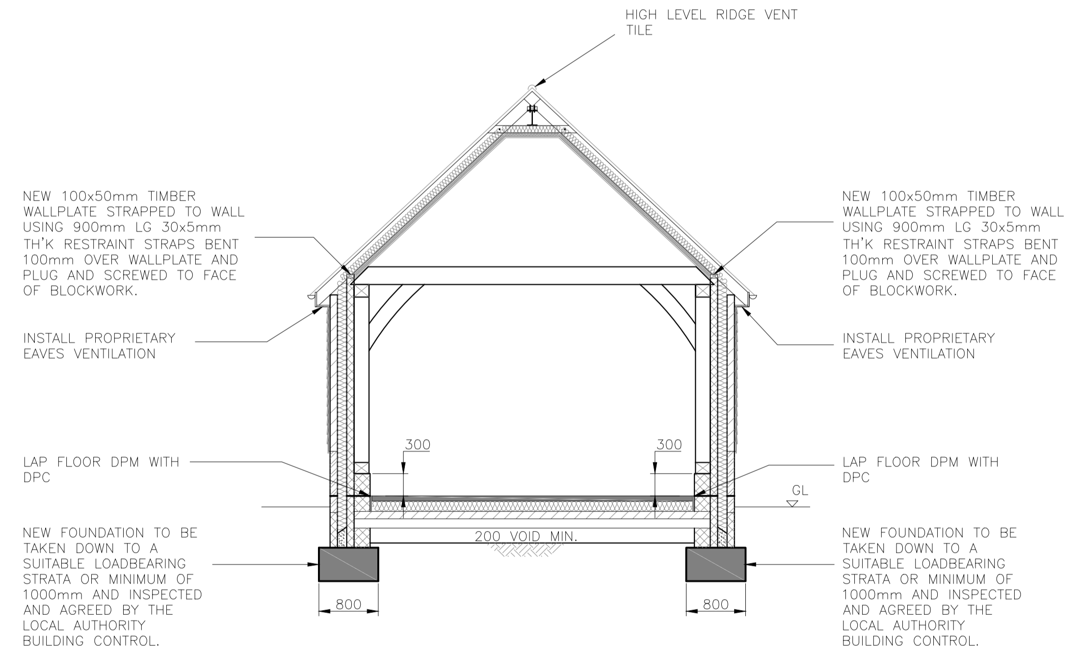
SECTION D-D SCALE 1:50
