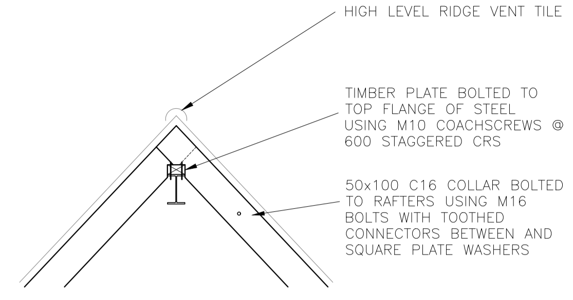
RIDGE DETAIL SCALE 1:20
