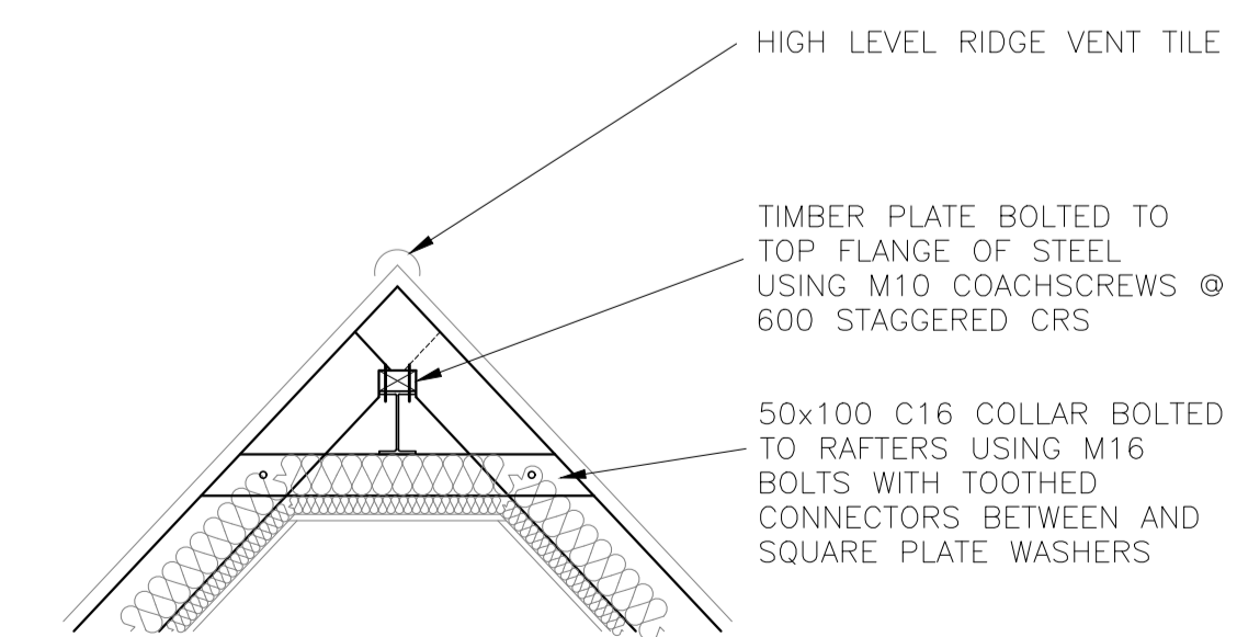
RIDGE DETAIL TO VAULTED ROOF SCALE 1:20
