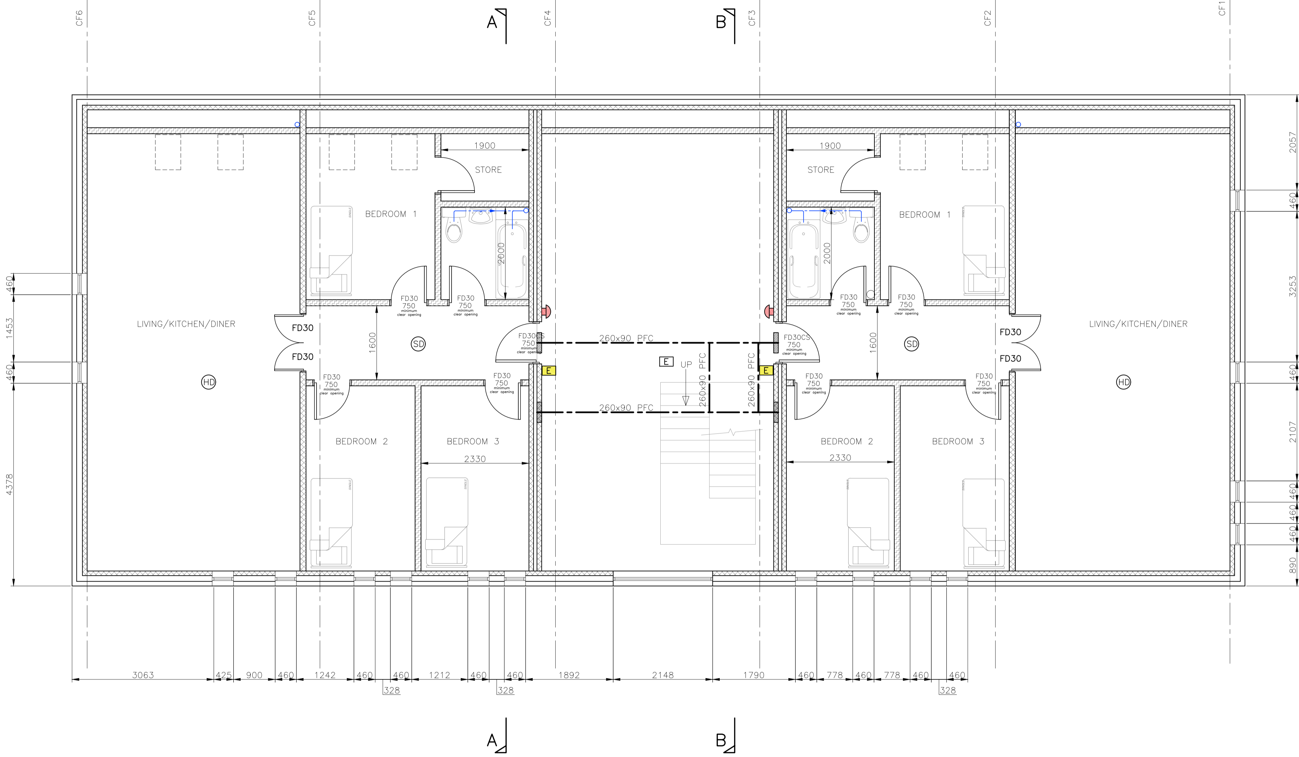
FIRST FLOOR LAYOUT SHOWING STEELWORK OVER SCALE 1:50
