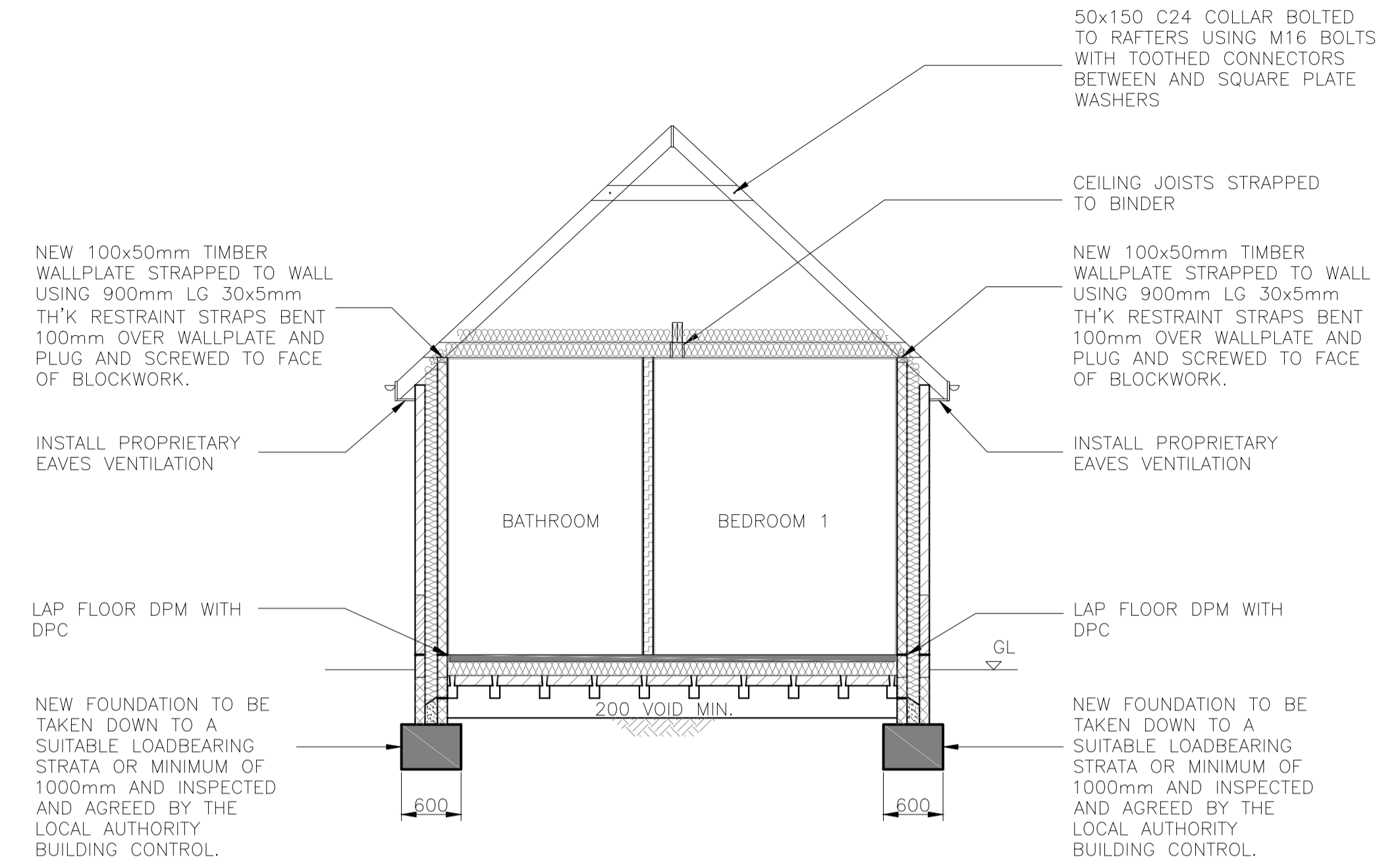
SECTION C-C SCALE 1:50
